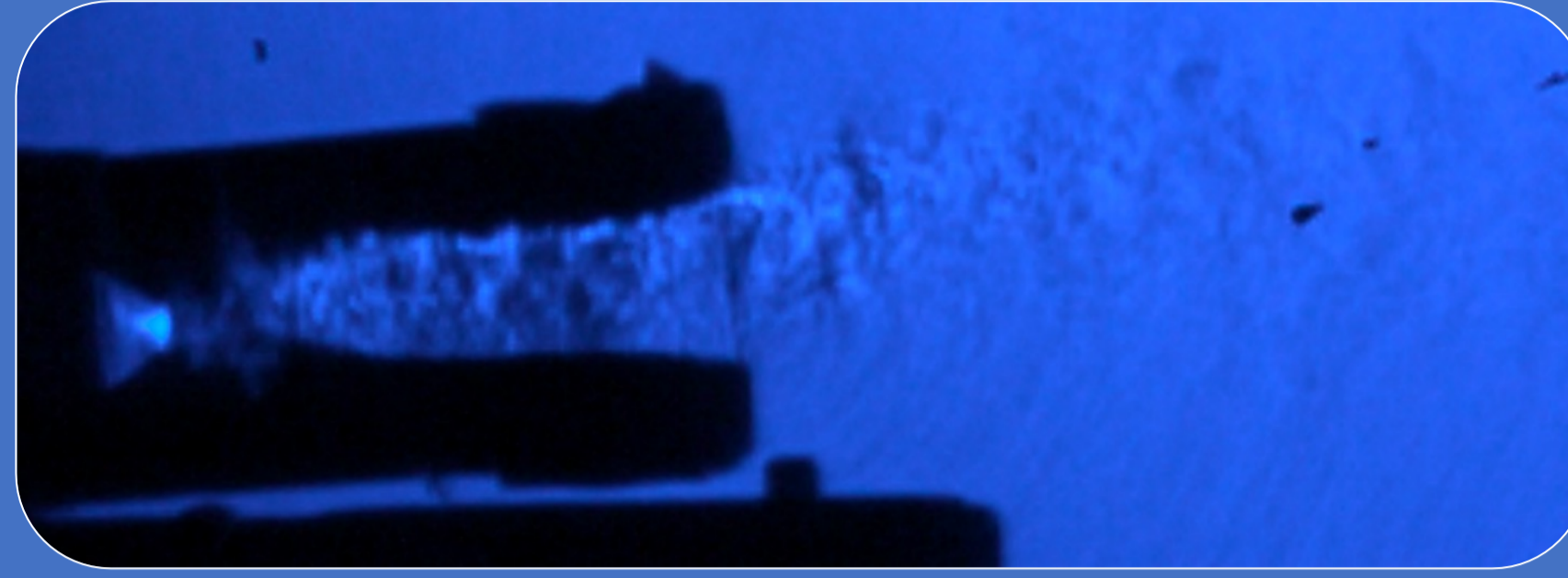
Image 2: Original Nozzle Design, Turbulent flow can be seen inside of the diverging section of the nozzle and flowing out of the exit.
